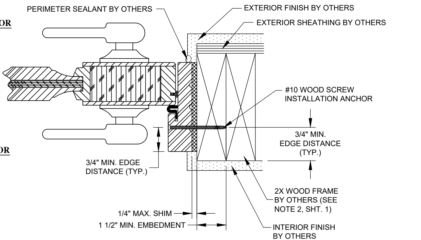
Q 11 HORIZONTAL SECTION WOOD FRAME SUBSTRATE STANDARD DESIGN JAMB FRAME
