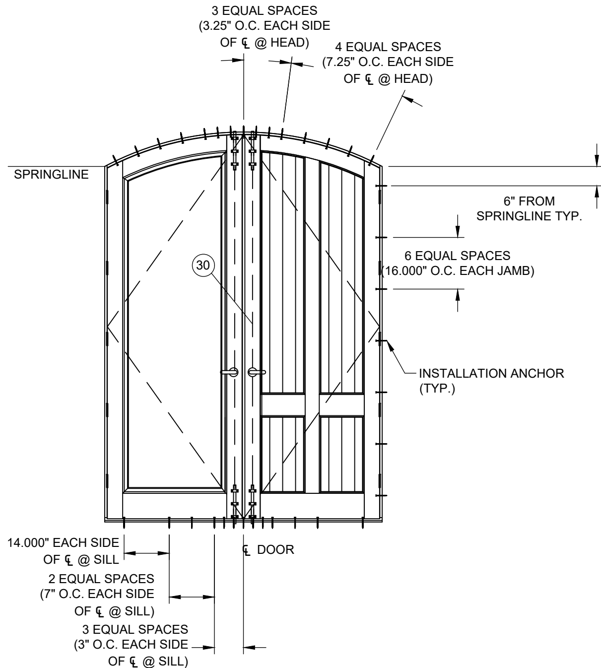
ANCHOR LAYOUT 3 INTERIOR VIEW (NOTE: NO INSTALLATION ANCHORS TO BE LOCATED CLOSER THAN 3" O.C.)
