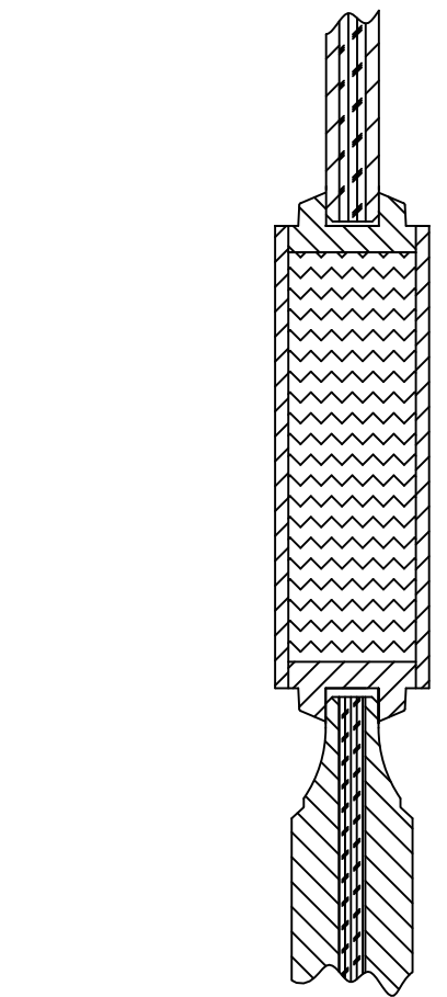
G 8 VERTICAL SECTION MEETING RAIL AND PANEL INSERTS
