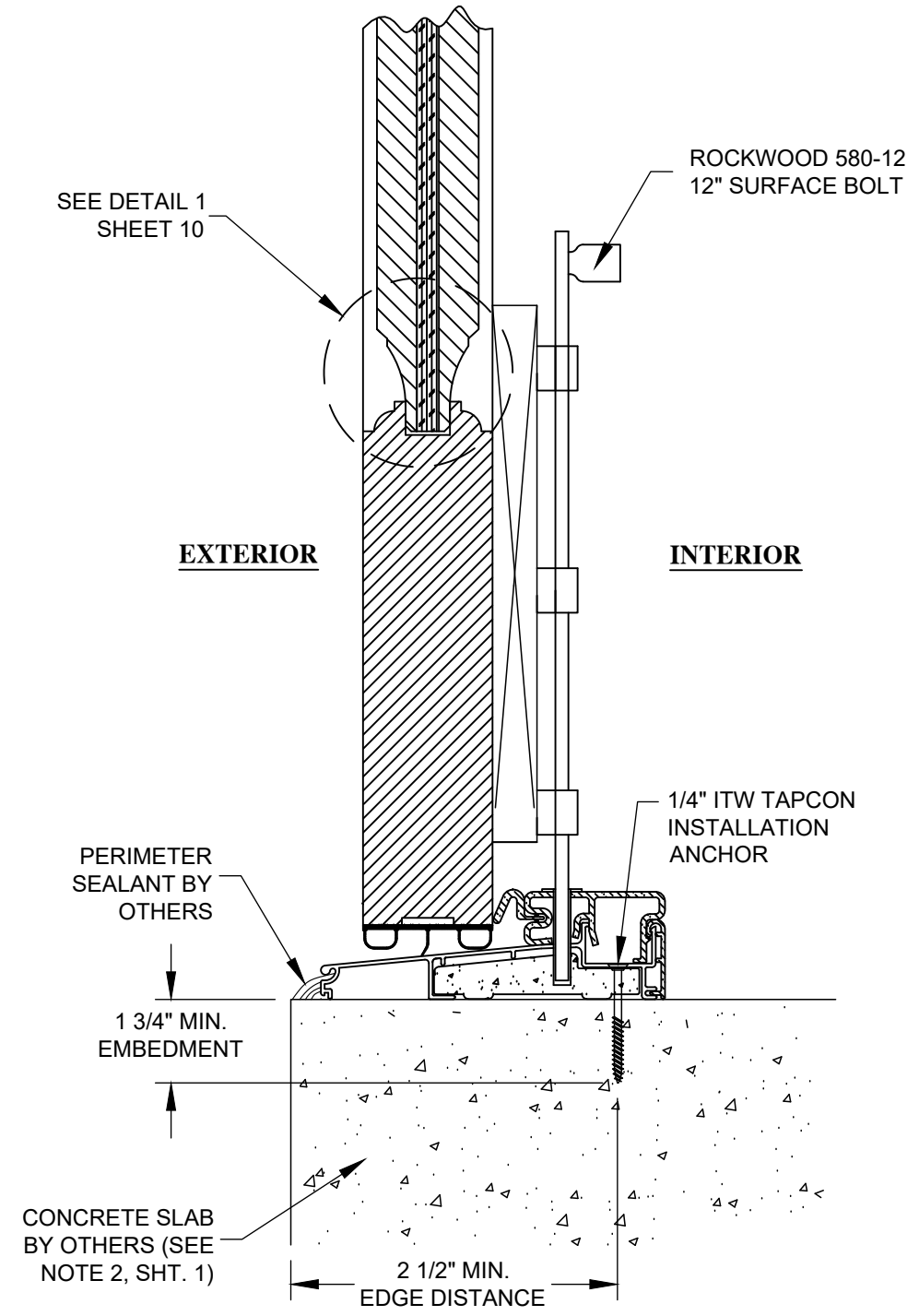
H 8 VERTICAL SECTION CONCRETE SUBSTRATE FLAT PANEL OR RAISED PANEL STANDARD DESIGN
