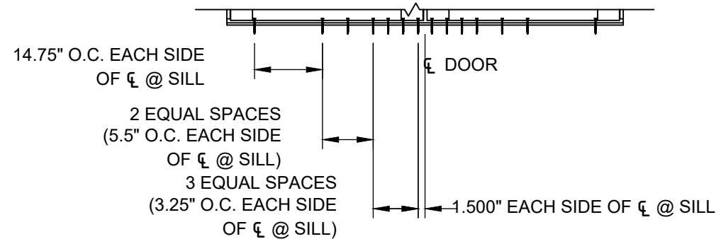
ANCHOR LAYOUT 3 FOR ALUMINUM THRESHOLD
