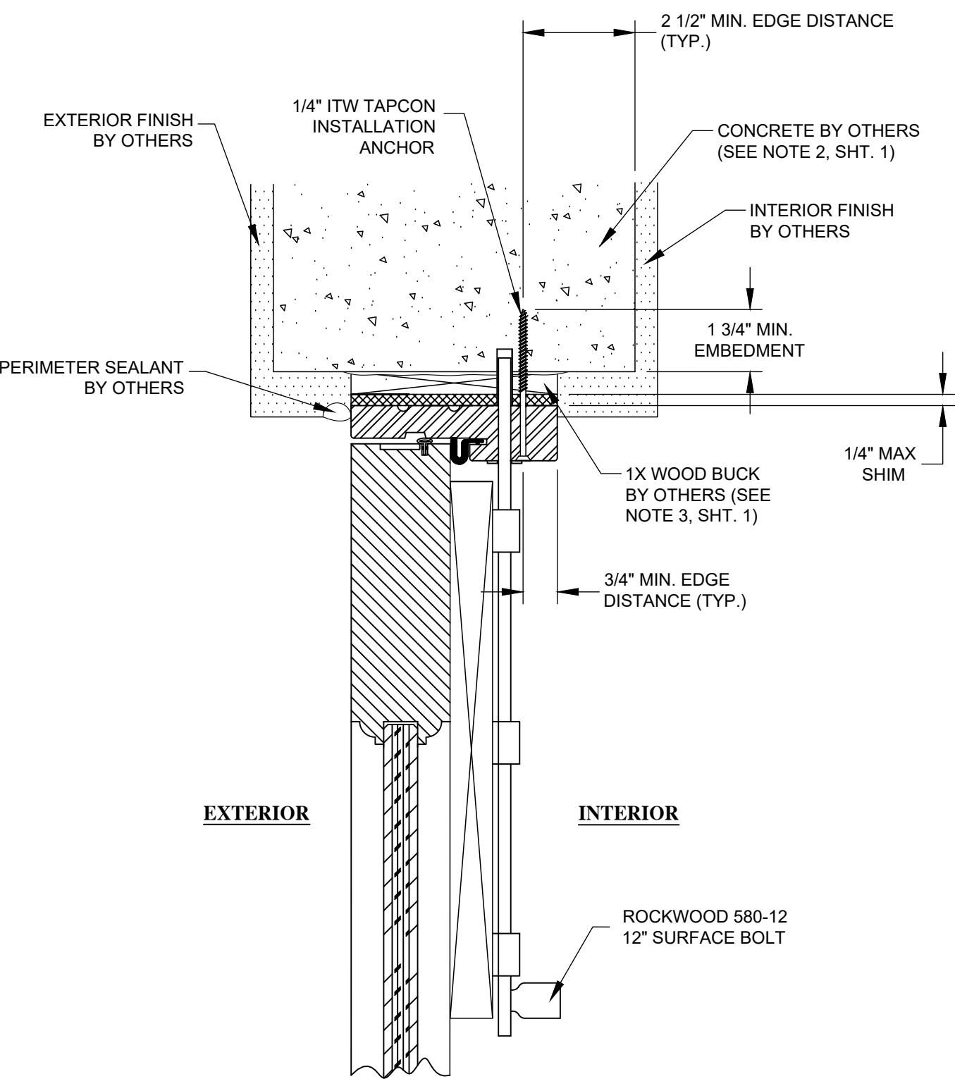
C VERTICAL SECTION 7 CONCRETE SUBSTRATE EURO DESIGN
