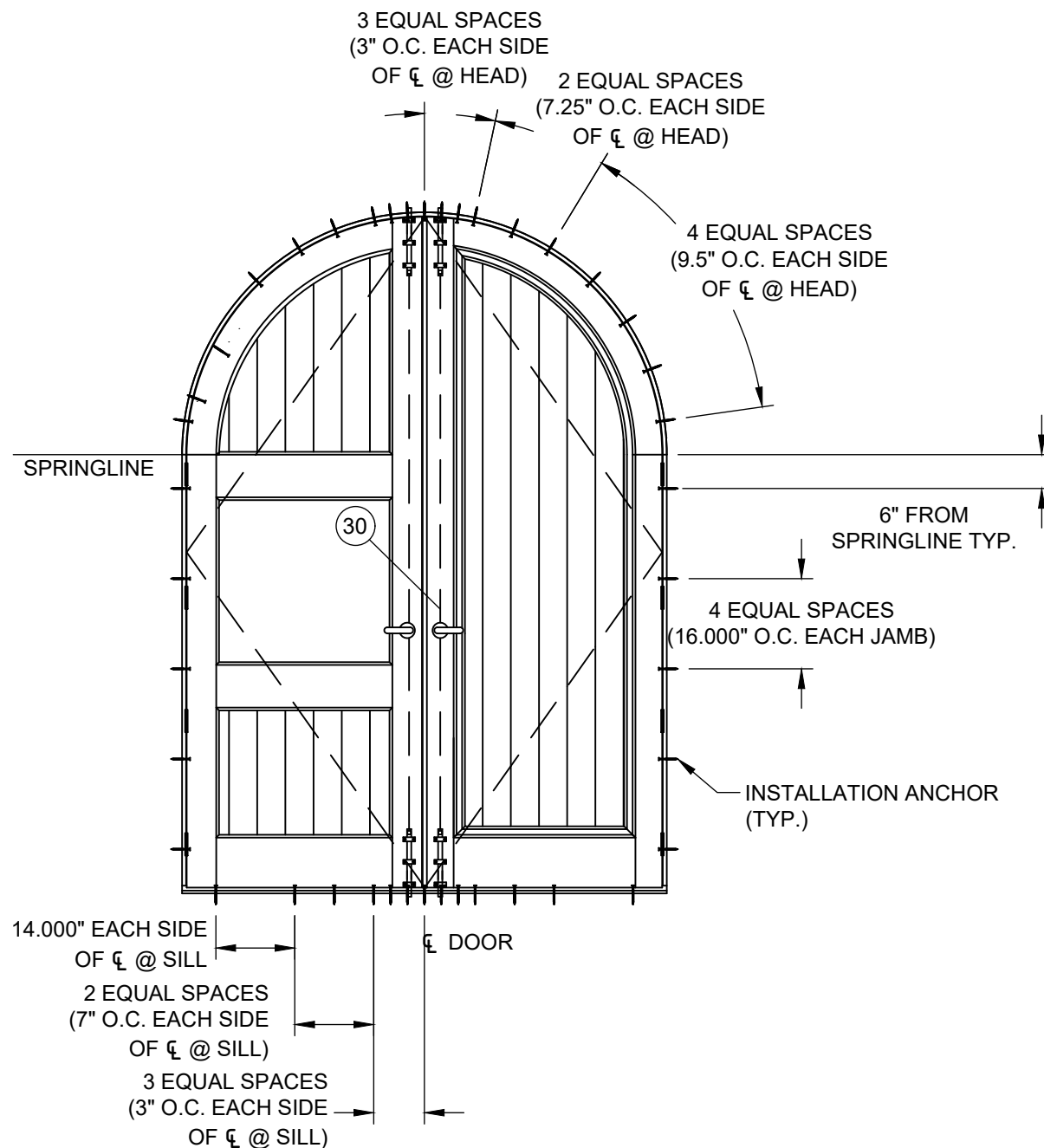
ANCHOR LAYOUT 2
