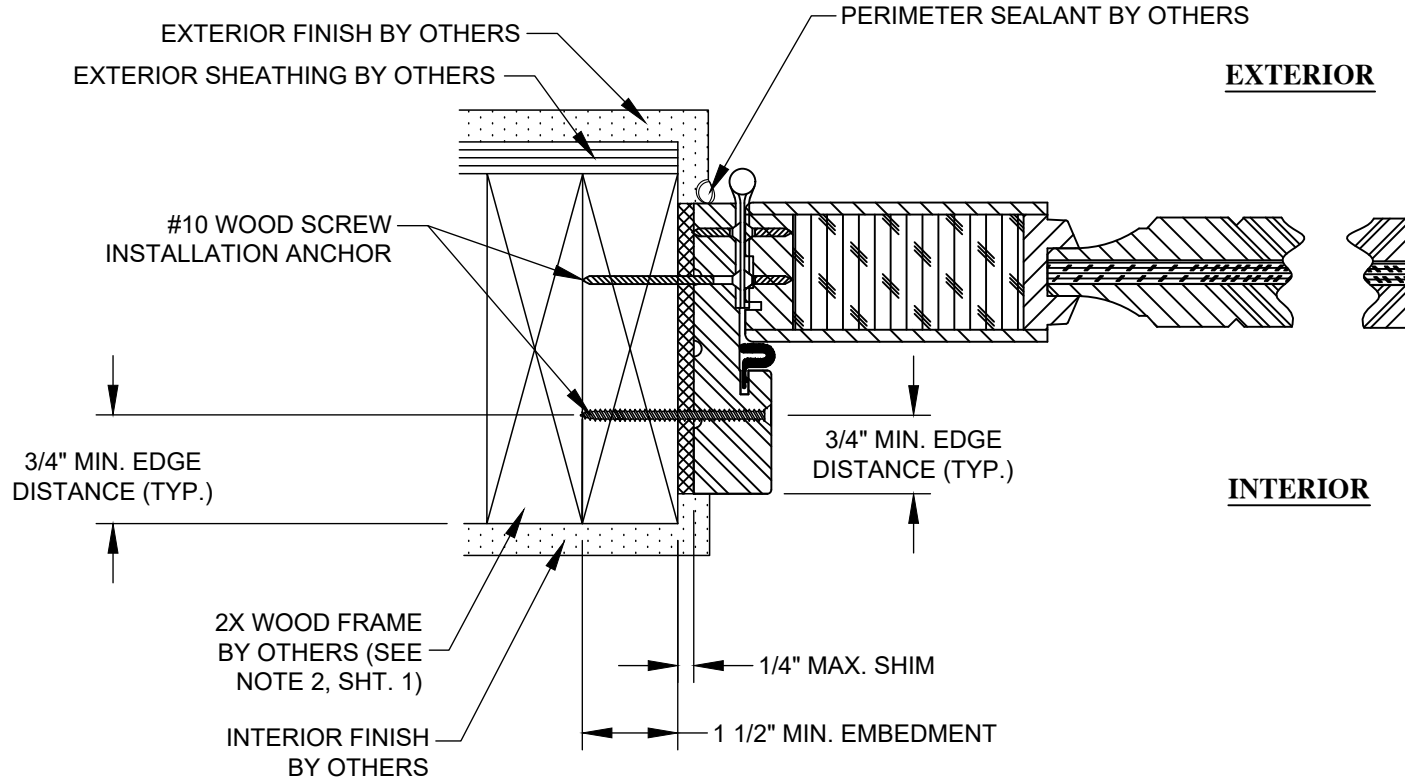
P 11 HORIZONTAL SECTION WOOD FRAME SUBSTRATE STANDARD DESIGN JAMB FRAME
