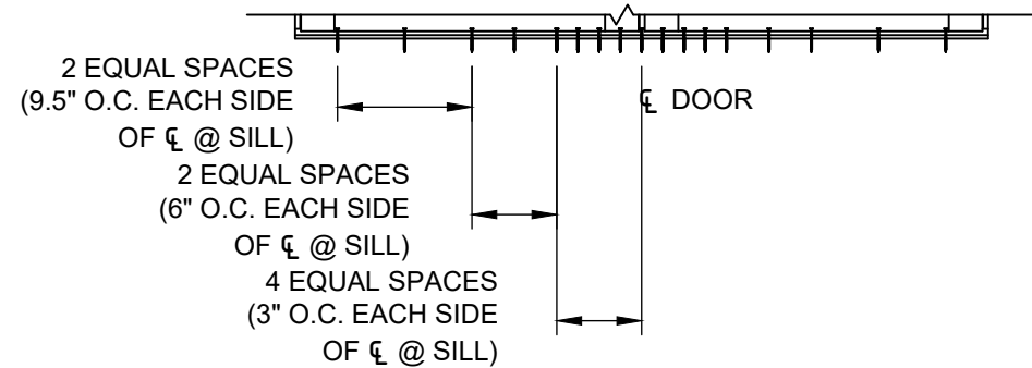
ANCHOR LAYOUT 4 FOR ALUMINUM THRESHOLD
