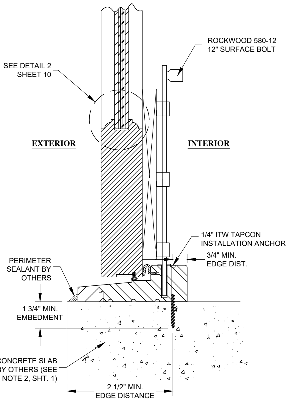
F 8 VERTICAL SECTION CONCRETE SUBSTRATE FLAT PANEL OR RAISED PANEL EURO DESIGN
