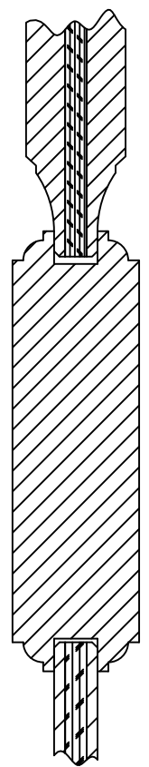
D VERTICAL SECTION 7 INTERMEDIATE RAIL AND PANEL INSERTS
