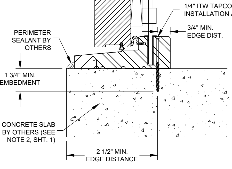
A VERTICAL SECTION 6 CONCRETE SUBSTRATE EURO DESIGN
