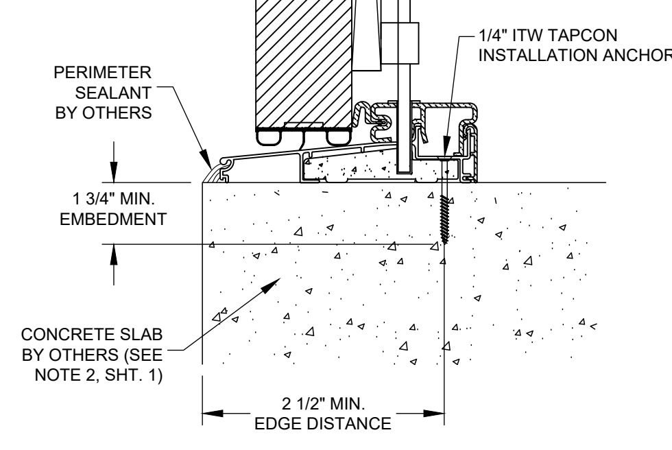
B VERTICAL SECTION 6 CONCRETE SUBSTRATE STANDARD DESIGN
