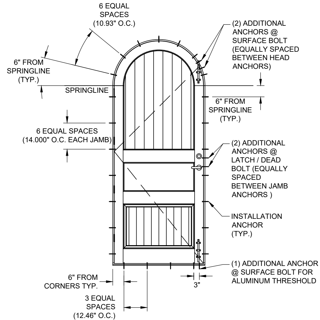
ANCHOR LAYOUT 1 INTERIOR VIEW
