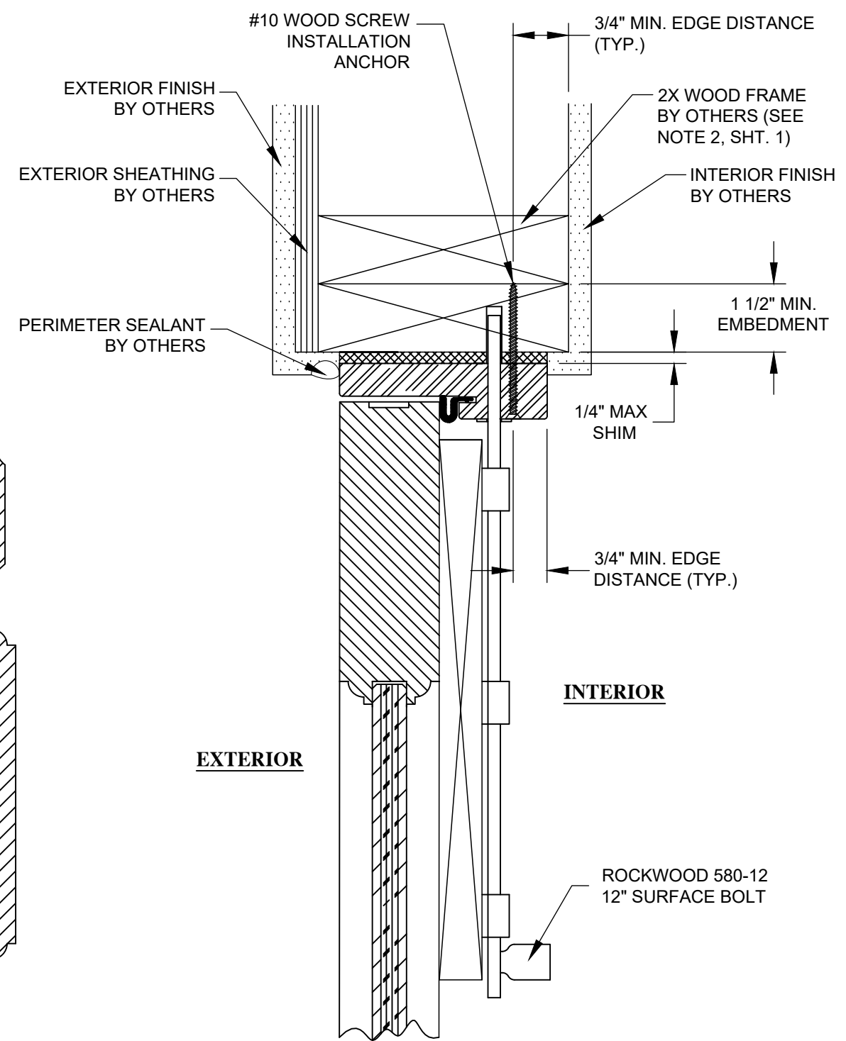
D VERTICAL SECTION 7 INTERMEDIATE RAIL AND PANEL INSERTS
